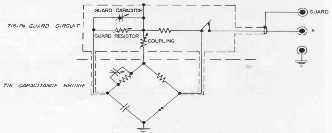
Figure 3. Elementary schematic circuit diagram of the Type 716-P4 Guard Circuit connected to the Type 716-C Capacitance Bridge.
