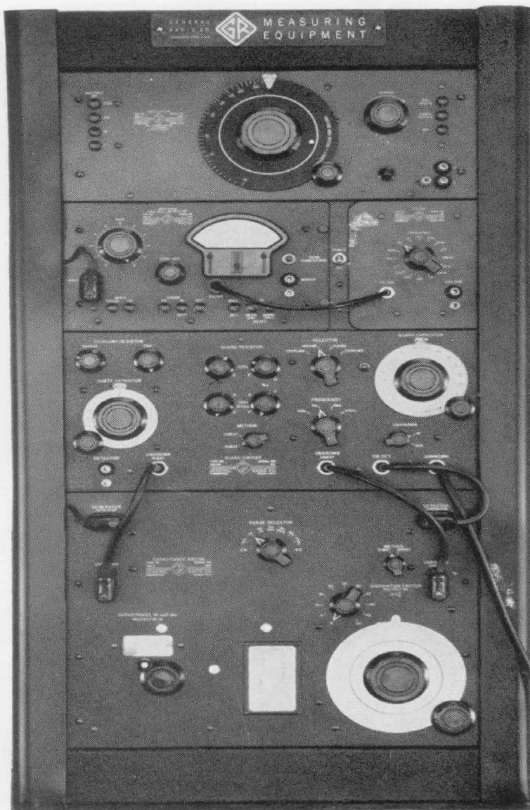
Figure 4. View of the Type 1610-A Capacitance Measuring Assembly consisting of guard circuit and bridge mounted in a relay-rack with associated equipment: Type 1302-A Oscillator, Type 1231-BRFA Amplifier and Null Detector, Type 716-P4R Guard Circuit, and Type 716-C Capacitance Bridge. Assembly includes relay rack and all necessary cables. Oscillator and amplifier operate from a 115-volt, 60 cycle power line.
