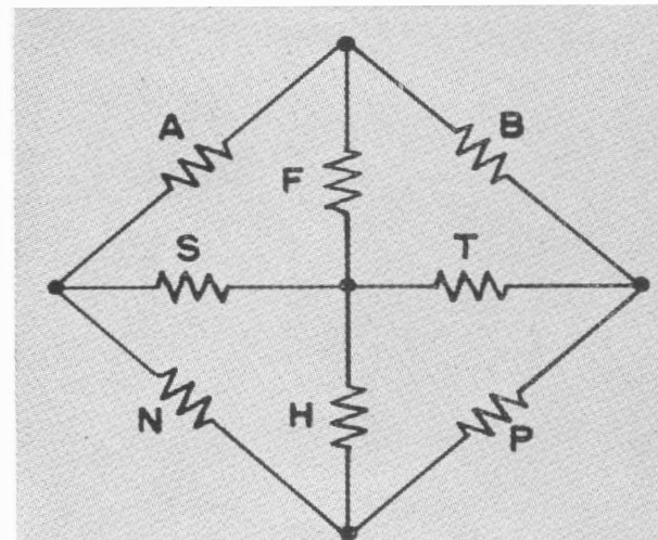
Figure 1. General bridge network with guard circuit.
