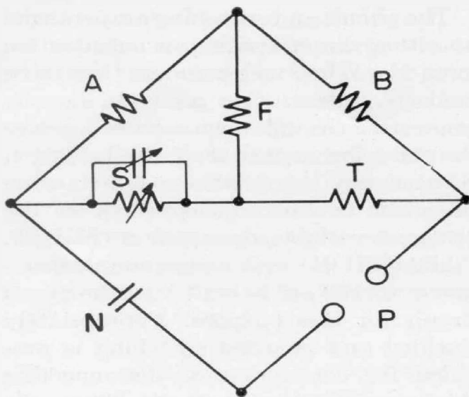
Figure 2. Basic schematic of bridge with guard circuit.
